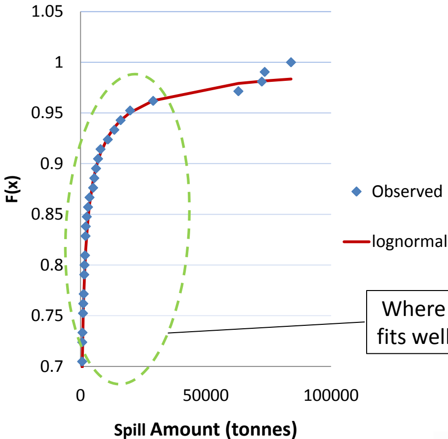
Lognormal
